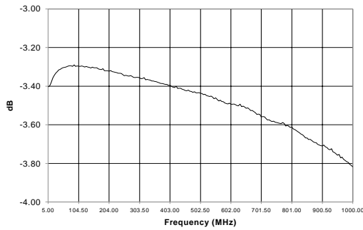
Amplitude Unbalance
